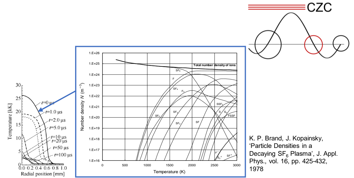
LTE concept
