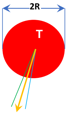
Net emission from the centre of an isothermal sphere
