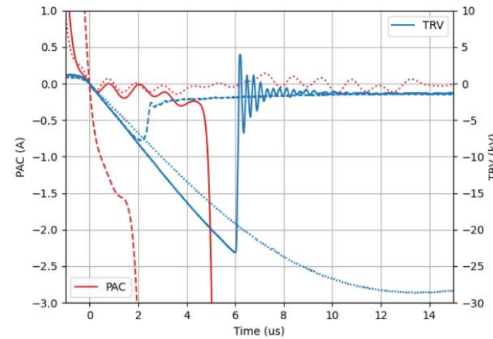
Fig. 3. Post-arc current and transient recovery voltage for success (dotted line), thermal failure (dashed line), and hot dielectric failure (solid line). All measurements performed in CO 2 /O 2 (90/10).
